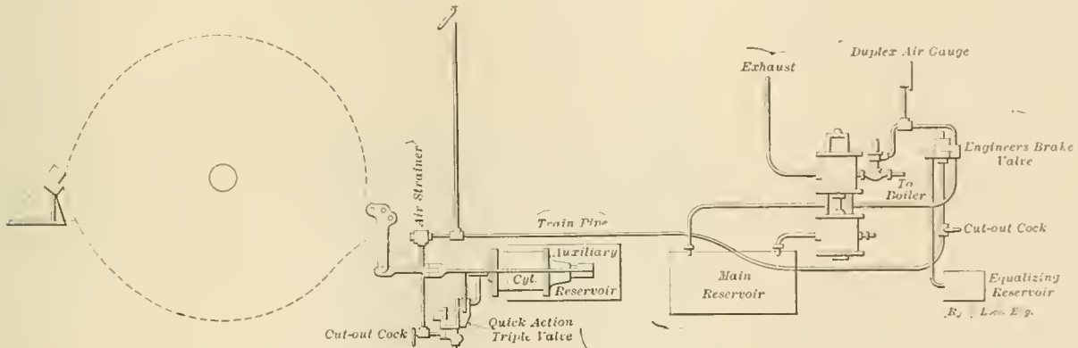
NOVEL APPLICATION OF THE AUTOMATIC BRAKE TO A MINE ENGINE HOISTING DRUM.
